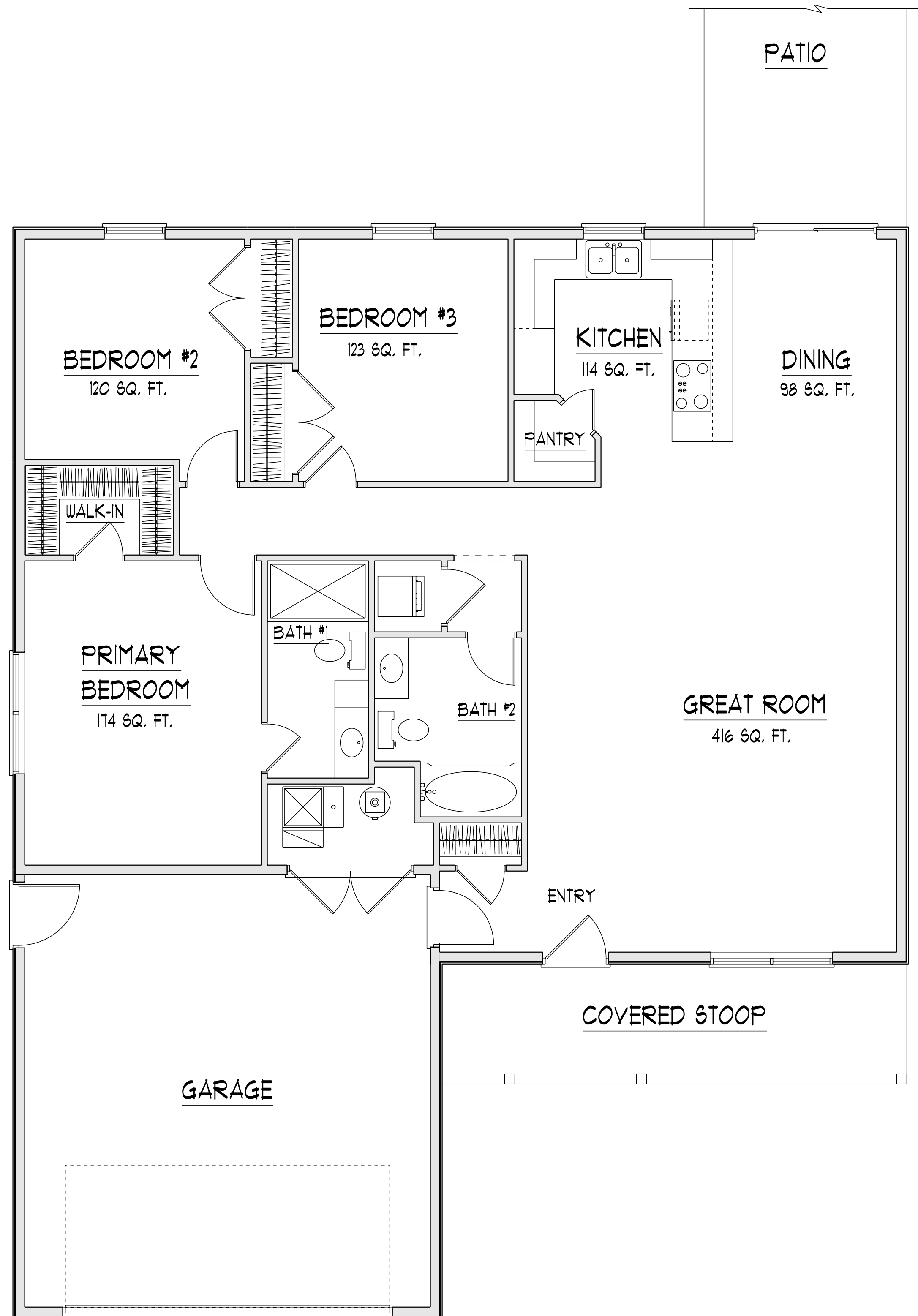
MAIN LEVEL FLOOR PLAN-"THE CREST"
