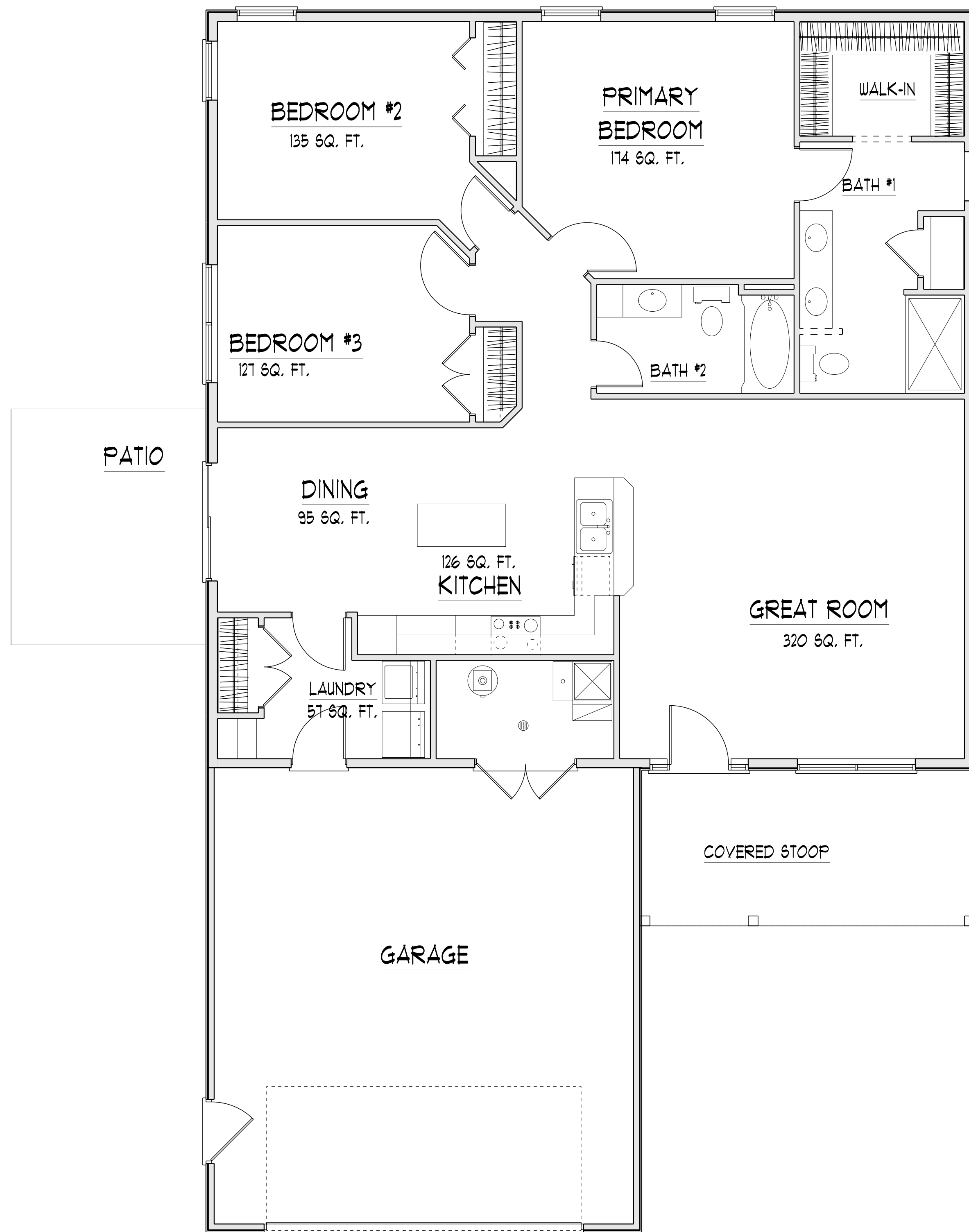
MAIN LEVEL FLOOR PLAN-"THE OVERLOOK"
